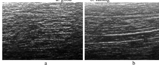
Figure 8 Photos of stretched side after bending a, INCONEL 825 b AISI 316L
