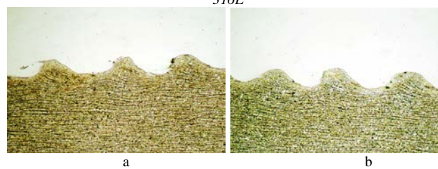
Figure 9 Microstructure of explosive welded bonds (interface)
