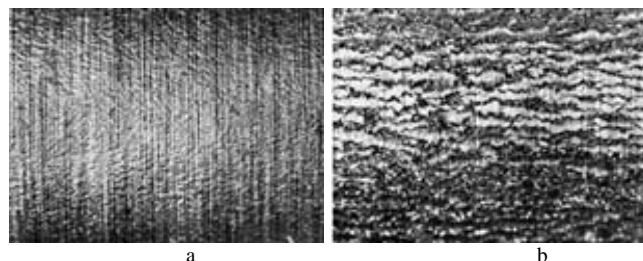
Figure 7 Referent photos of the stretched side of the bend spesimens a. good b. failing
