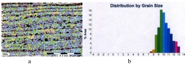
Figure 1 (a and b) Microstructure of base metal and grain size distribution
