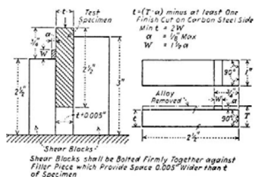
Figure 6 Preparation of specimens for shear test
