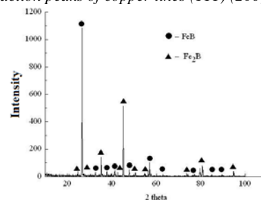
Fig. 3. Diffraction pattern taken from the surface steel 45 with boride coatings obtained after boriding at using EMF
