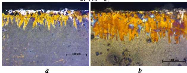
Fig. 6. Microstructures coatings on steel 45 obtained after complex saturation with boron and copper in different physical – chemical conditions: a – complex saturation with boron and copper without EMF, duration saturation – 4 hours, x200; b – complex saturation with boron and copper + EMF, saturation duration – 2 hours, x200 (color high temperature etching at 400 °C)
