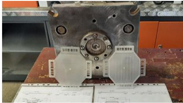
Fig. 4 Filter-drainage and turbulator, casting mold and molded plastic parts
