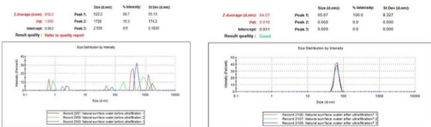
Fig. 8 Particle size in natural surface water before and after ultrafiltration
