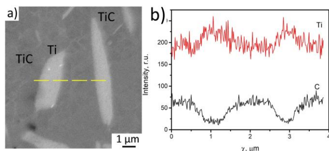
Fig.5. The microstructure of Ti-TiC after hot-presssing at 1500 °C (a) and distribution of chemical elements (b) though TiC-Ti-TiC-Ti particles yellow line in (a).
