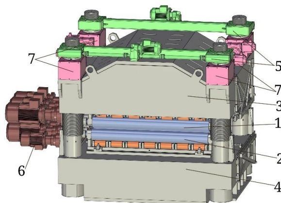
Fig. 1. Components of the roll leveler
