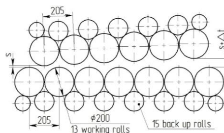
Fig. 2. Roll arrangement
