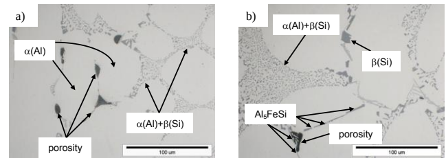
Fig. 5 Microstructure (LM) of AlSi7Mg alloy showing the causes of shrinkage porosity: a) at the grain boundaries of the \alpha(Al) solution; b) as a result of Al_5FeSi phase crystallization.
