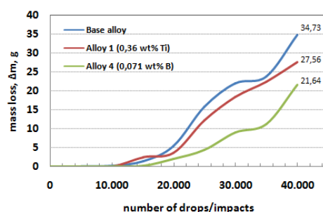
Figure 6. Resistance to repeated impacts of as-cast grinding balls
