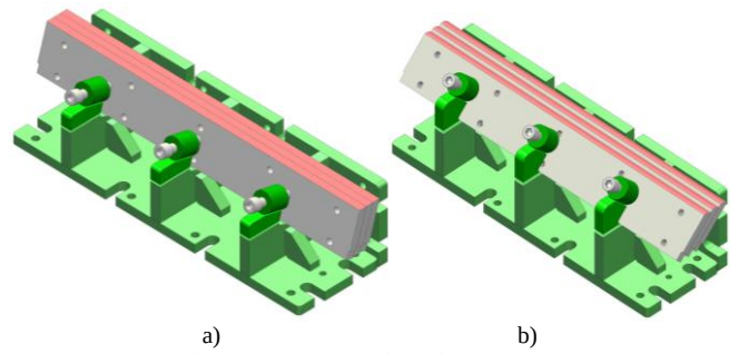
Fig. 4. Fixtures for machining chamfers of Blade I and Blade II parts. a) Fixture I, for milling a chamfer with an angle of 15^\circ , b) Fixture II, for milling a chamfer with an angle of 45^\circ
