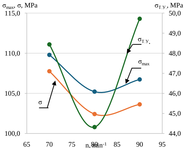
Fig. 2 – The effect of the screw rotation frequency of the extruder on tensile strength ( \sigma_{max} ), fracture strength ( \sigma ), and conditional yield strength ( \sigma_{T.y.} ) for PCM CPA-6-20
