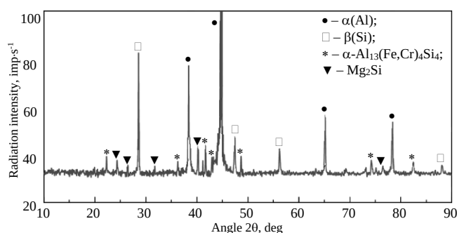
Fig. 4 XRD pattern of AlSi7Mg alloy with chromium addition.
