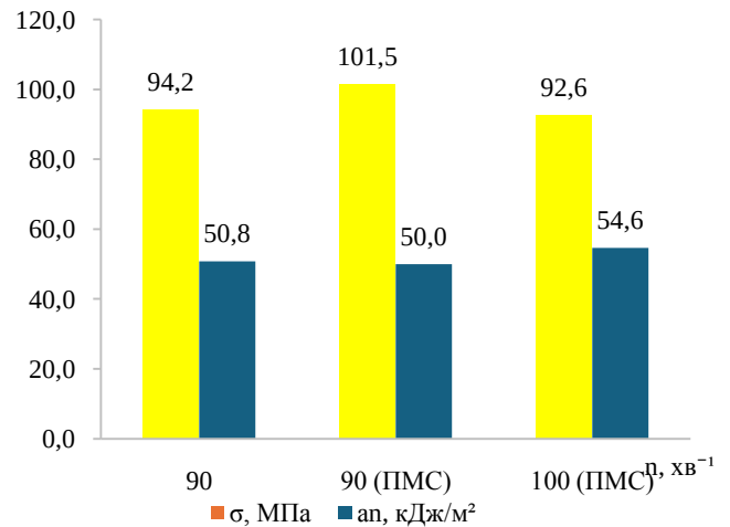
Fig. 3 – The effect of the screw rotation frequency of the extruder and the introduction of PMS-400 lubricant into the PCM composition on the yield stress and impact toughness of the resulting material.
