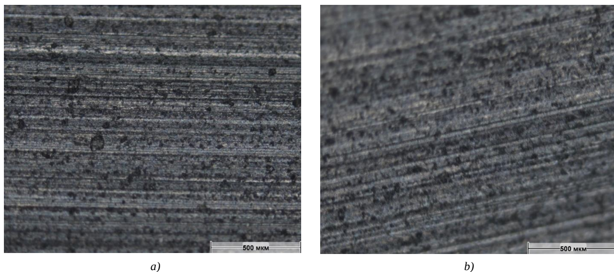
Fig. 2. The surface of the tip of the cutter \times 100 : a) basic; b) laser-treated
